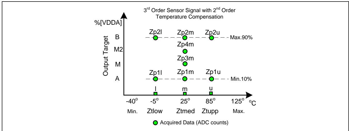
Figure 2.3 Calibration Points and Target Values for Sensor Measurements
