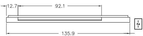
TOP VIEW OF CELL (M8:1)
