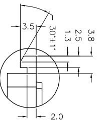
DETAIL C
