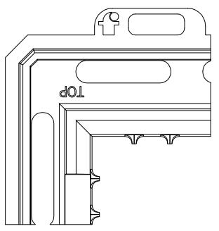
DETAIL S SCALE 4:1
