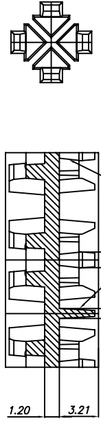
VACUUM CELL (SCALE:5/1)
