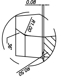
DETAIL "G" (SCALE:10/1)
