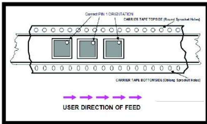
For Square BGA/QFN/COL/WLCSP Packages
