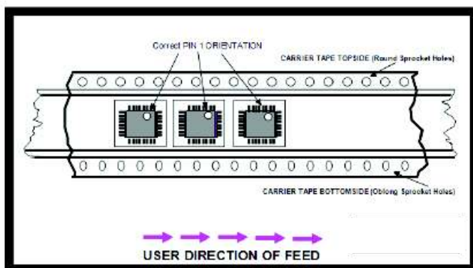
For Square 4-Side Leaded Packages
