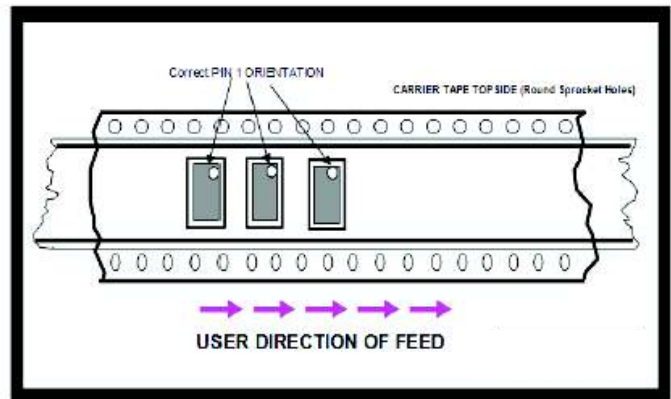
For Rectangular BGA/QFN/COL/WLCSP Packages
