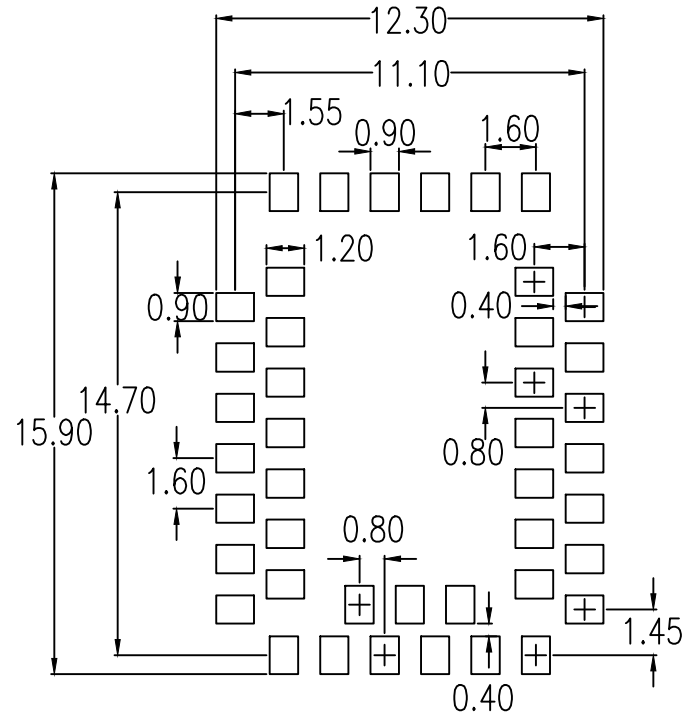
LAND PATTERN DIMENSION
