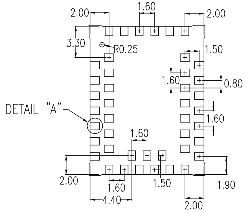
BOTTOM VIEW
