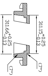
SECTION B - B(1:1)
