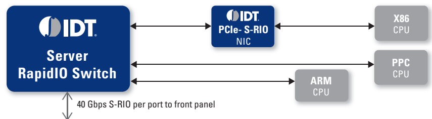
Heterogeneous MEC board block diagram.
